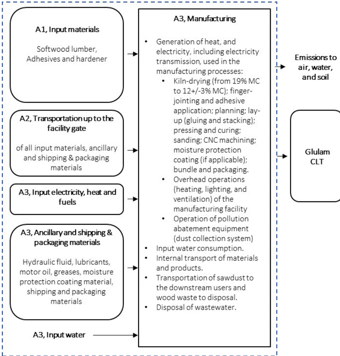
Figure 3 Production stage (module A1 to A3) system boundary of Element5 Glulam manufacturing
