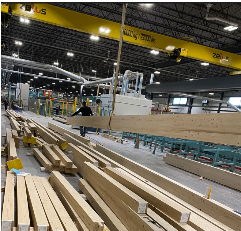
Figure 2 Element5 Glulam manufacturing line
